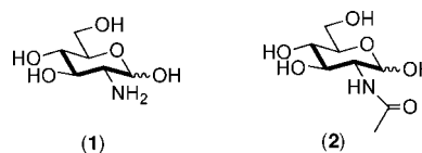
Figure 1. Glucosamine (1) and N -acetyl glucosamine (2).
